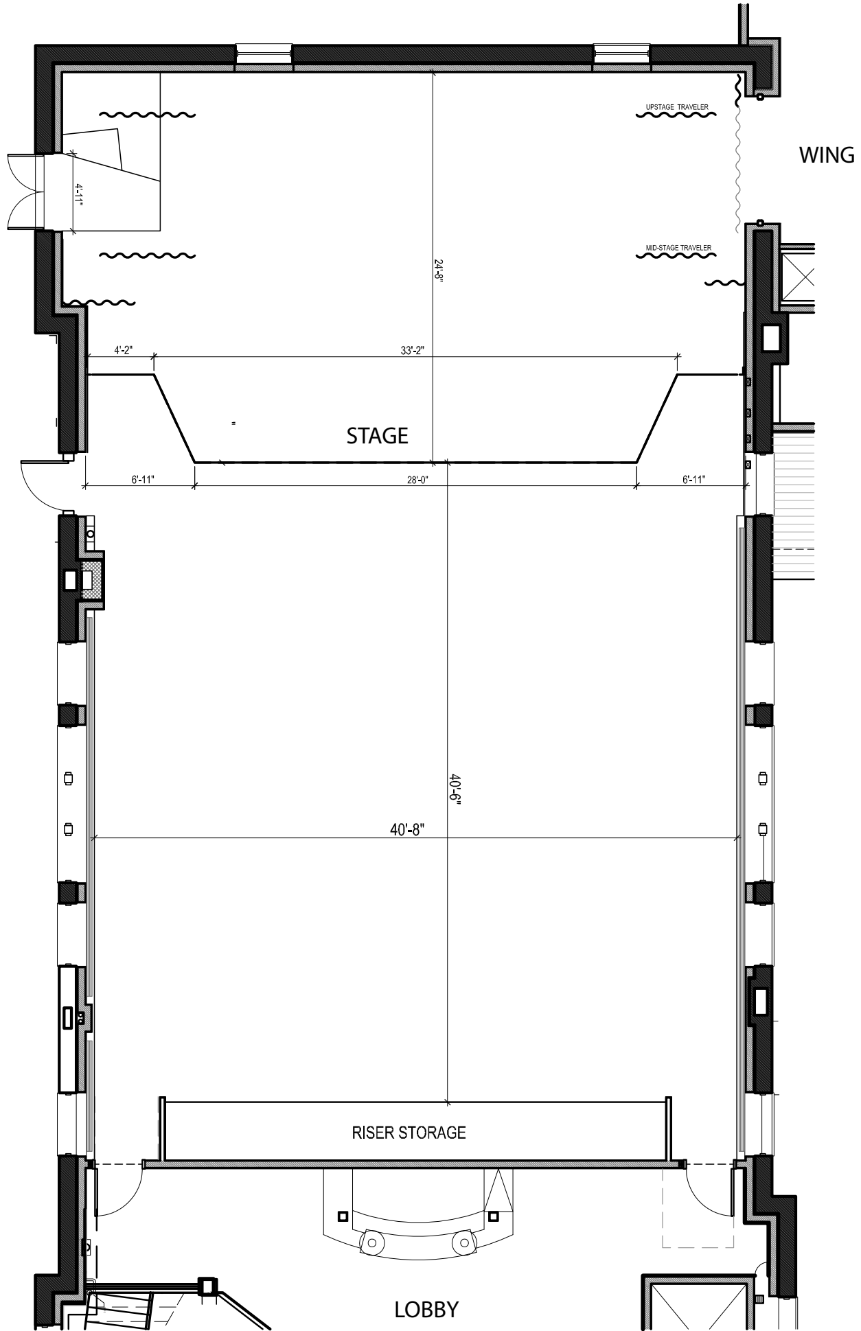
Volkert Main Stage - House Floor Plan
